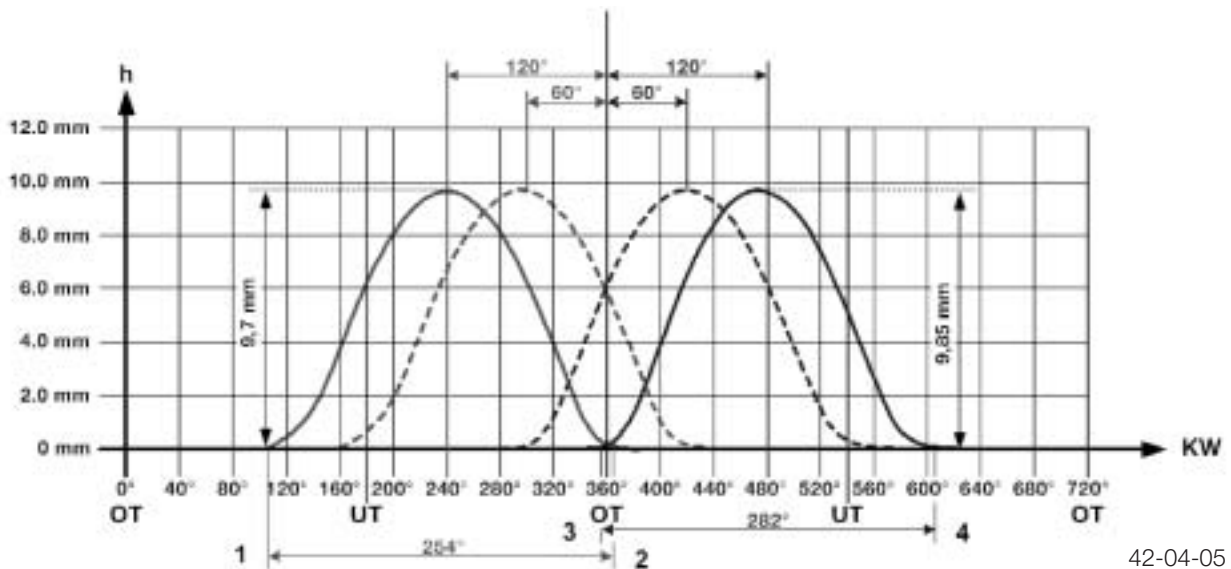
Exhaust & Intake Valve
